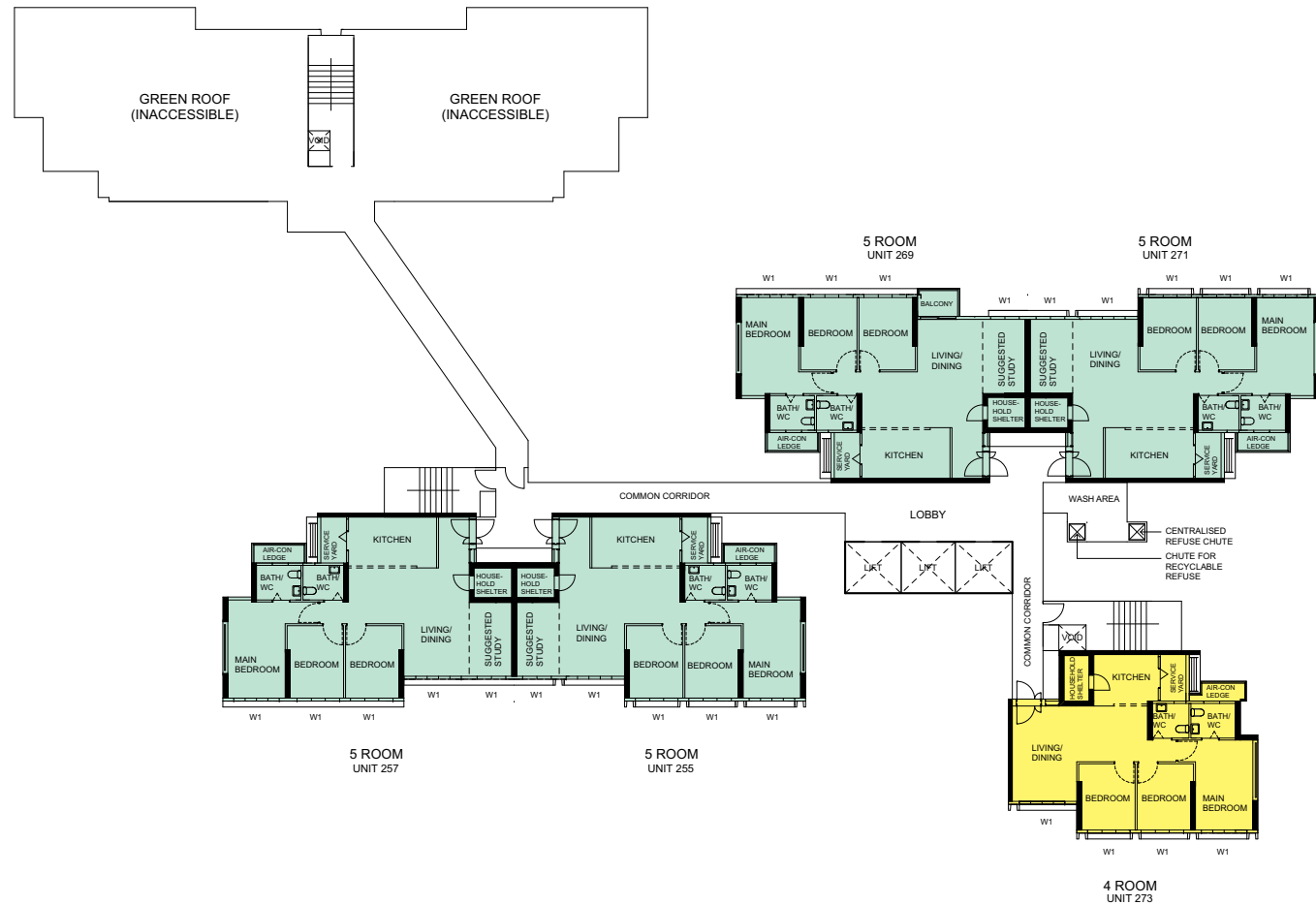
BLOCK 210C (18TH STOREY FLOOR PLAN)
