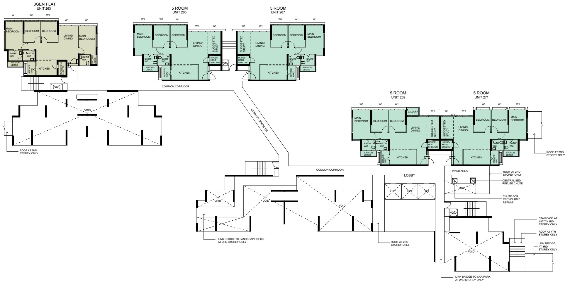
BLOCK 210C (3RD STOREY FLOOR PLAN)
