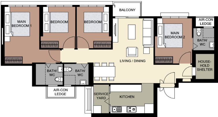
LAYOUT IDEAS FOR 3GEN FLAT APPROX. FLOOR AREA 123 sqm (Inclusive of Internal Floor Area of 118 sqm and Air-Con Ledges)
